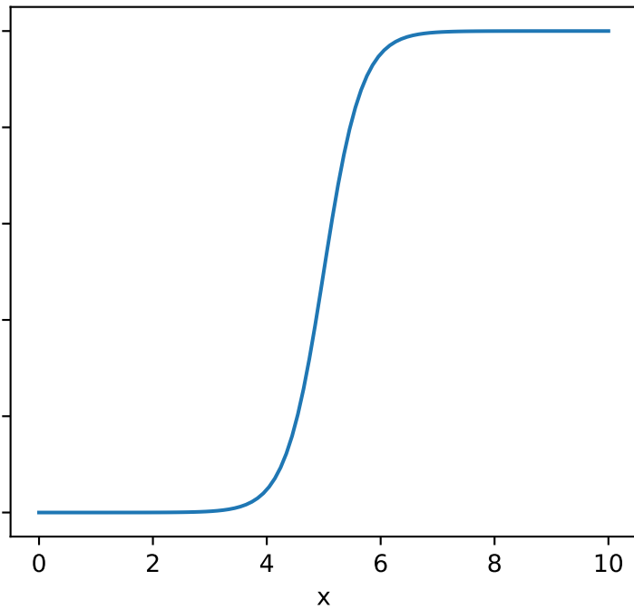
Beta = 3
