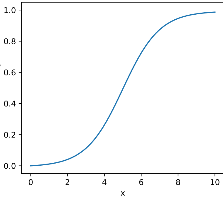
Beta = 1
