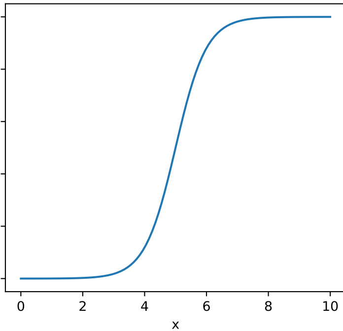
Beta = 2
